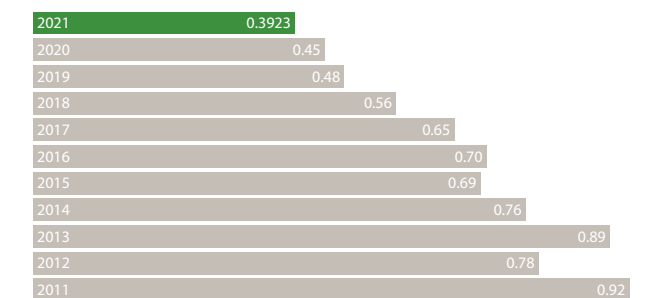
Nitrogen Oxide Emissions per Ton of Cement Clinker from 2011 to 2021 Unit: kg/ton
